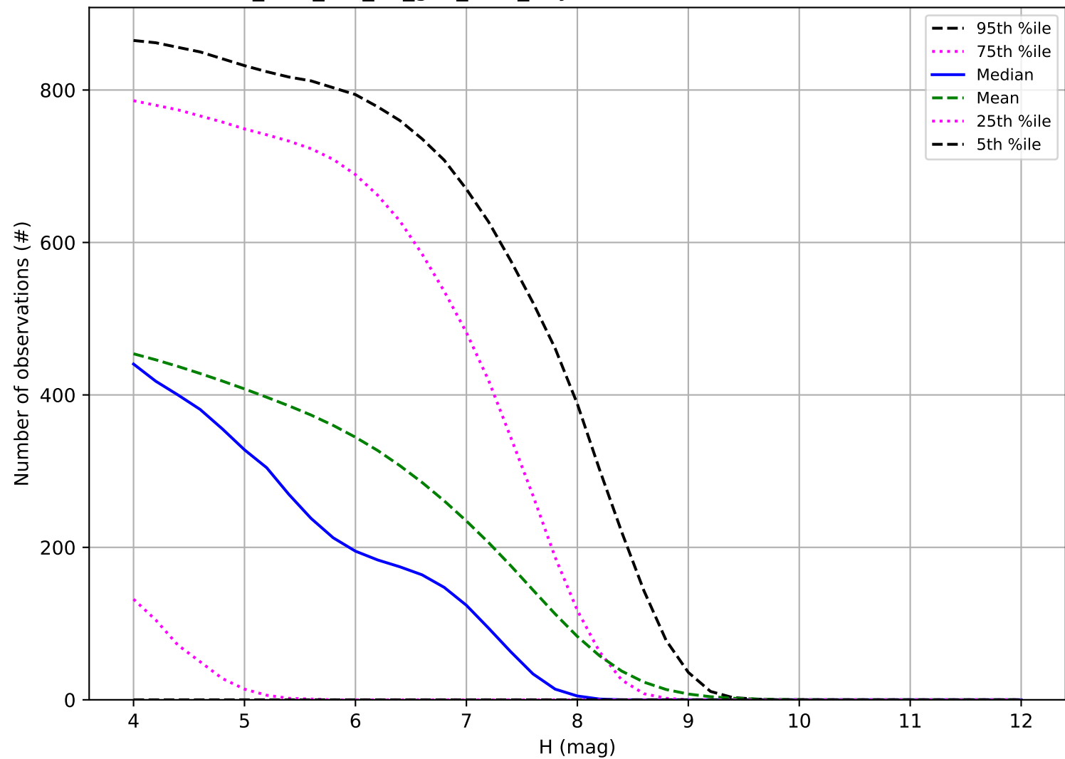
too_elab_r64_d2_griz_v3.4_10yrs: Number of observations TNO
