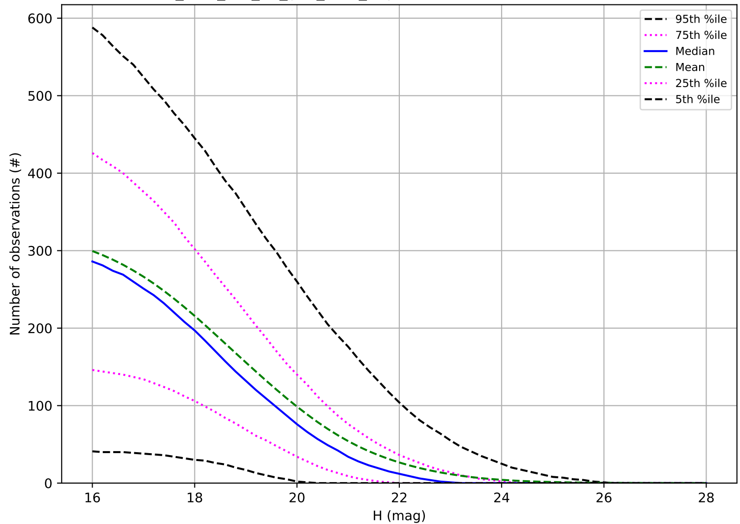
too_elab_r64_d2_griz_v3.4_10yrs: Number of observations PHA
