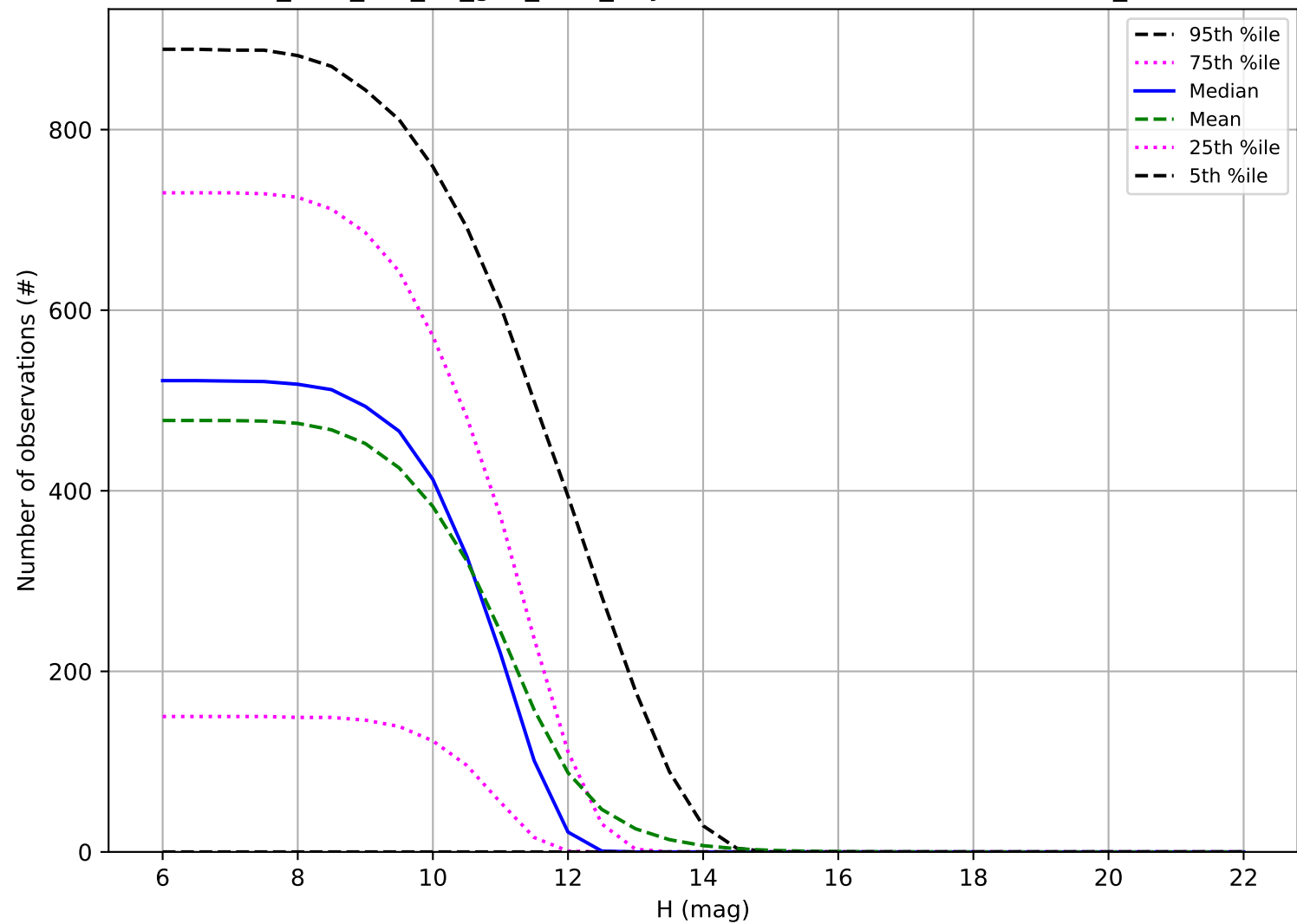
too_elab_r64_d2_griz_v3.4_10yrs: Number of observations OCC_r20
