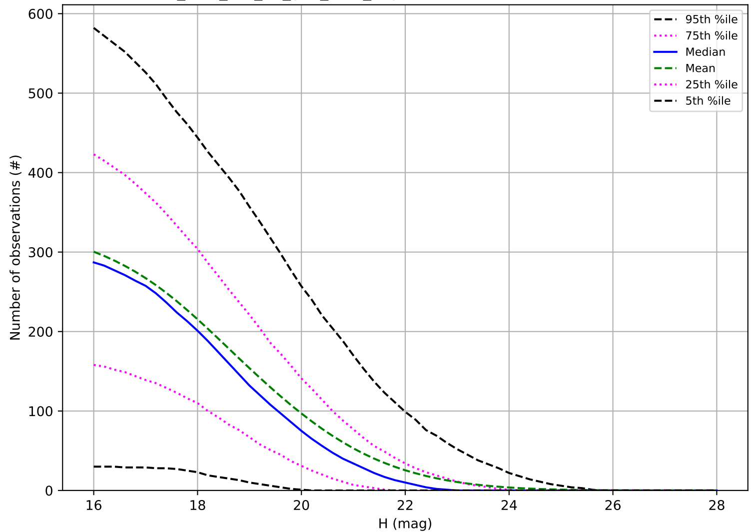
too_elab_r64_d2_griz_v3.4_10yrs: Number of observations NEO
