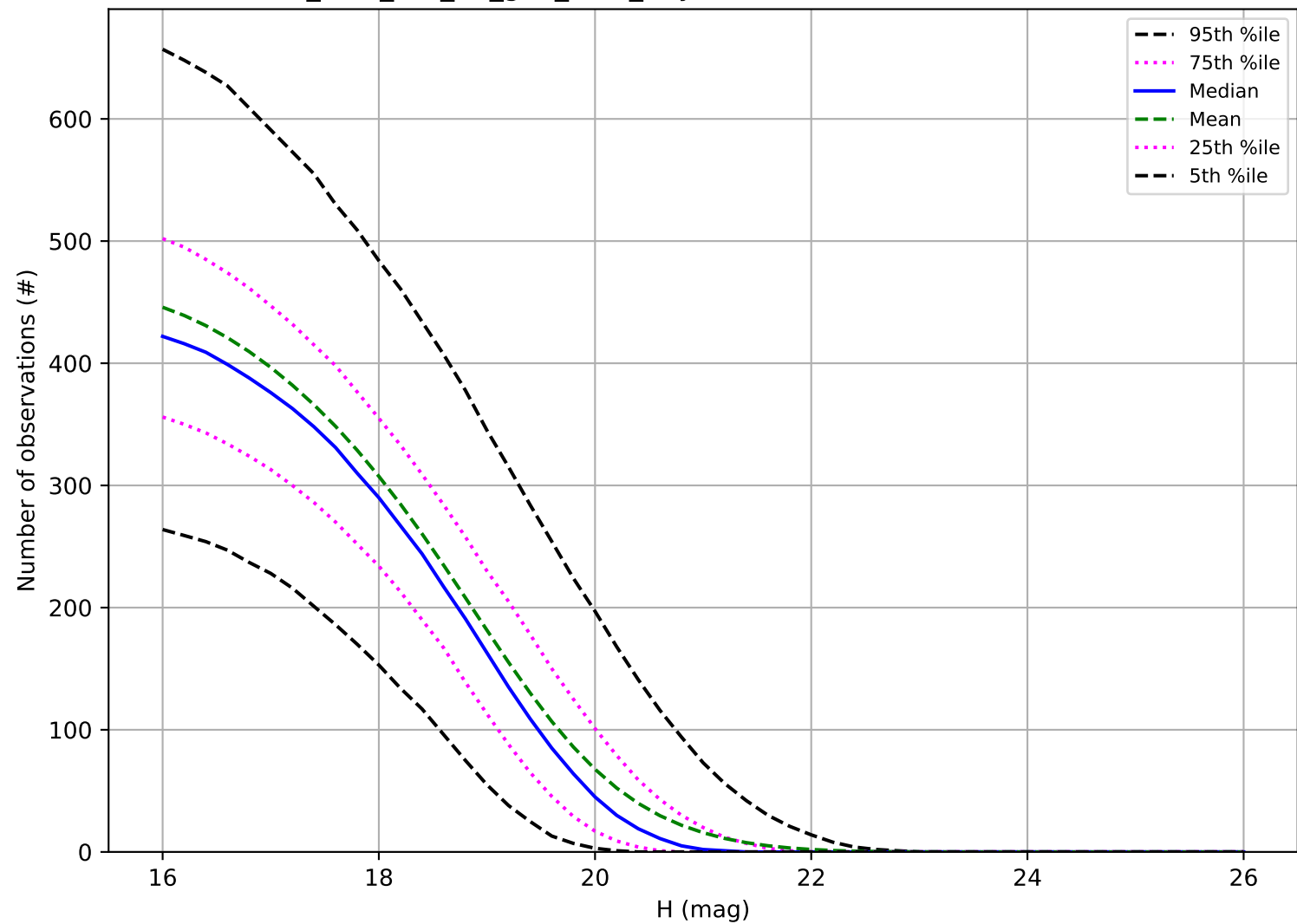
too_elab_r64_d2_griz_v3.4_10yrs: Number of observations MBA
