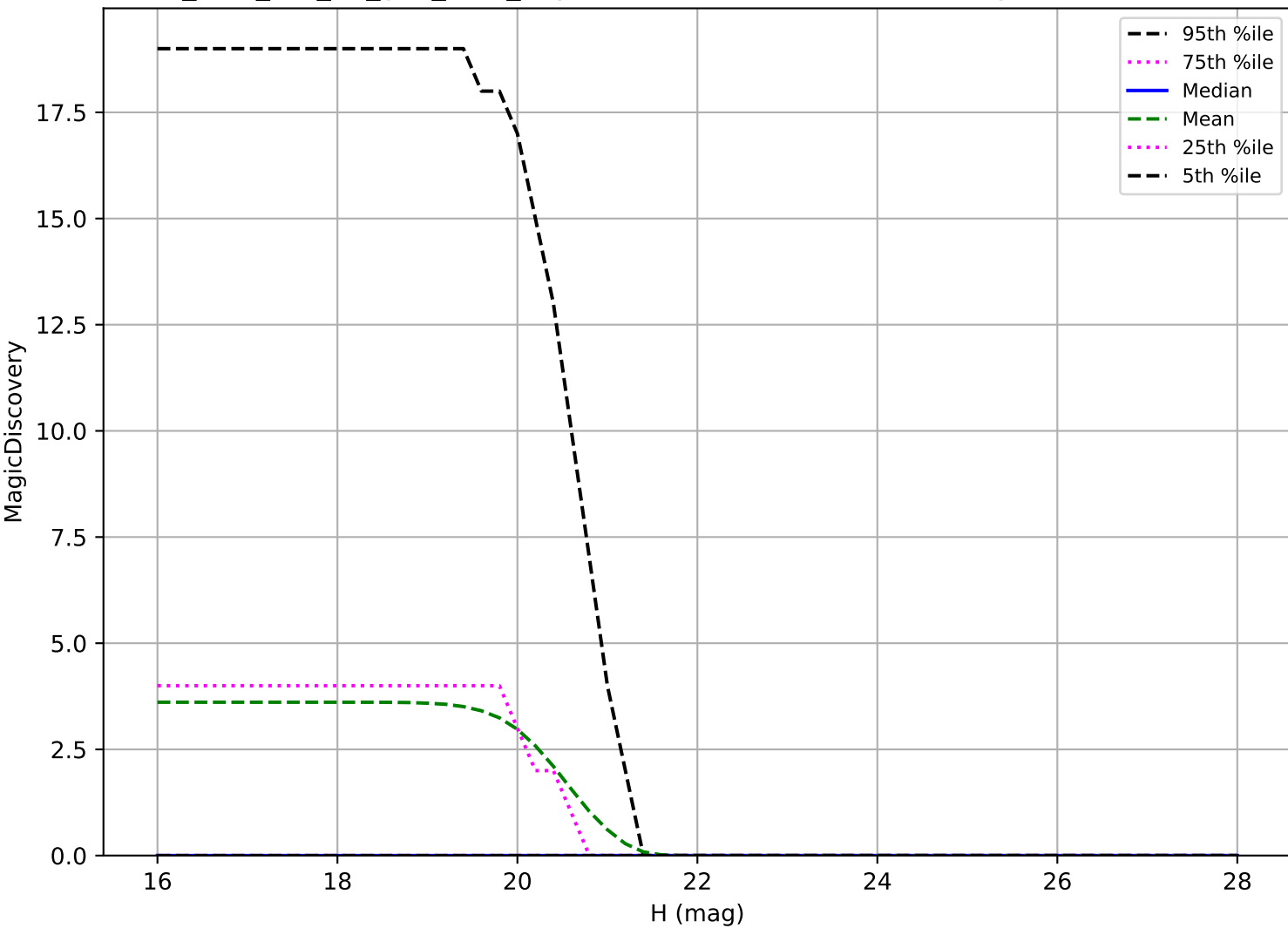
too_elab_r64_d2_griz_v3.4_10yrs: Vatira 6 detections in 60 nights detection loss
