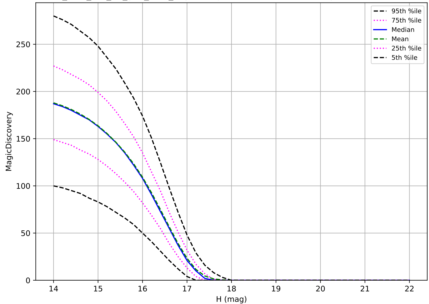
too_elab_r64_d2_griz_v3.4_10yrs: Trojan 6 detections in 60 nights detection loss
