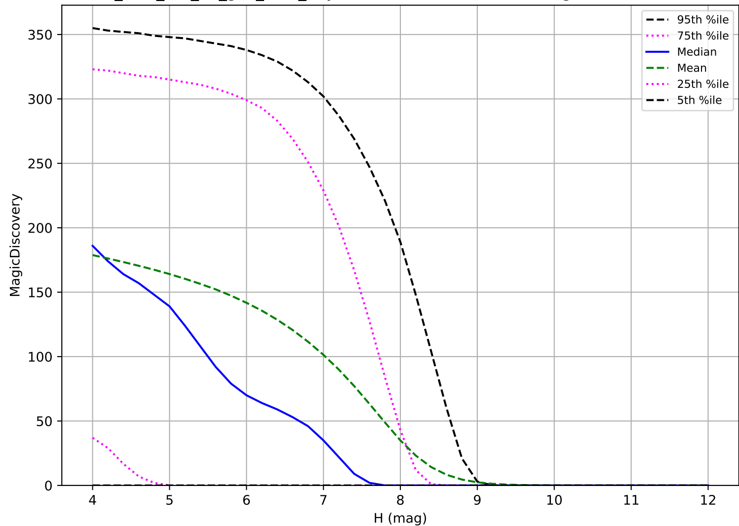
too_elab_r64_d2_griz_v3.4_10yrs: TNO 6 detections in 60 nights detection loss
