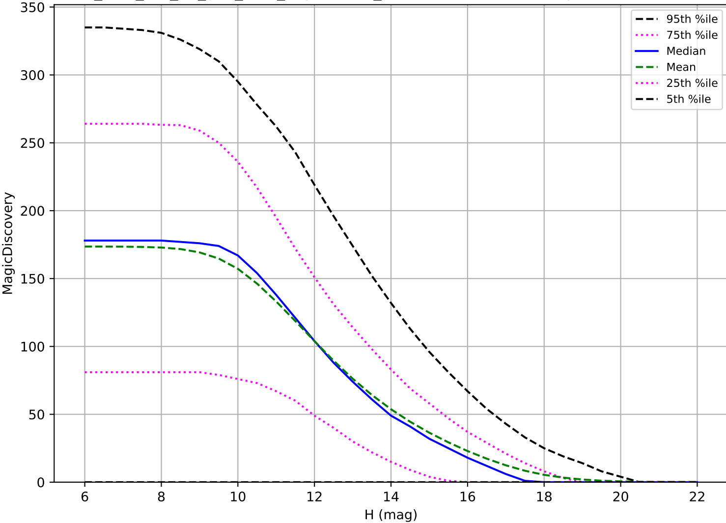
too_elab_r64_d2_griz_v3.4_10yrs: OCC_r5 6 detections in 60 nights detection loss
