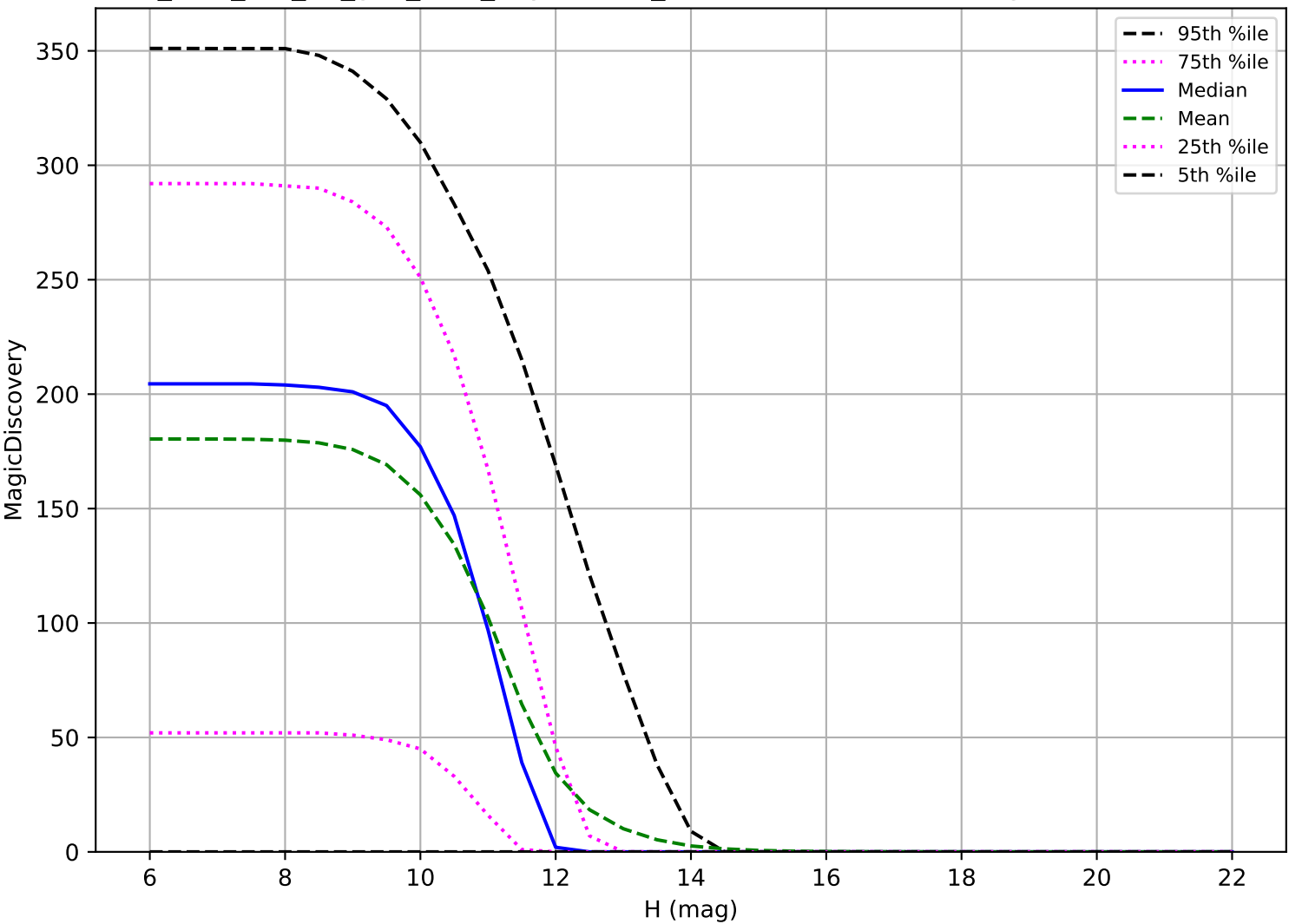
too_elab_r64_d2_griz_v3.4_10yrs: OCC_r20 6 detections in 60 nights detection loss
