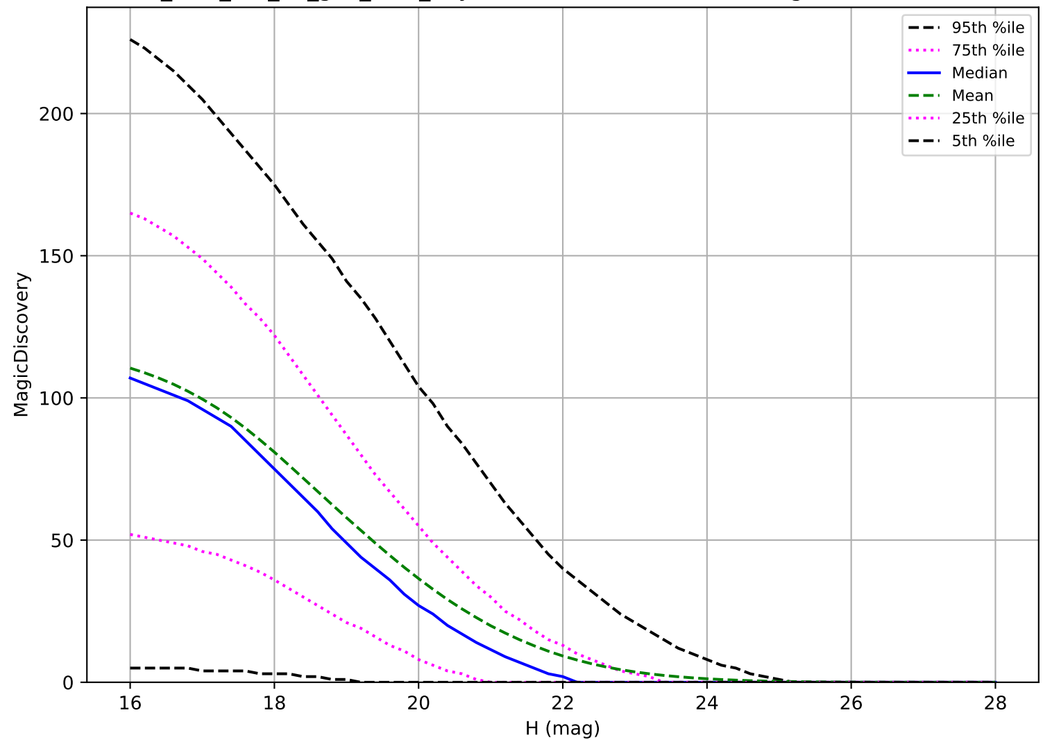
too_elab_r64_d2_griz_v3.4_10yrs: NEO 6 detections in 60 nights detection loss
