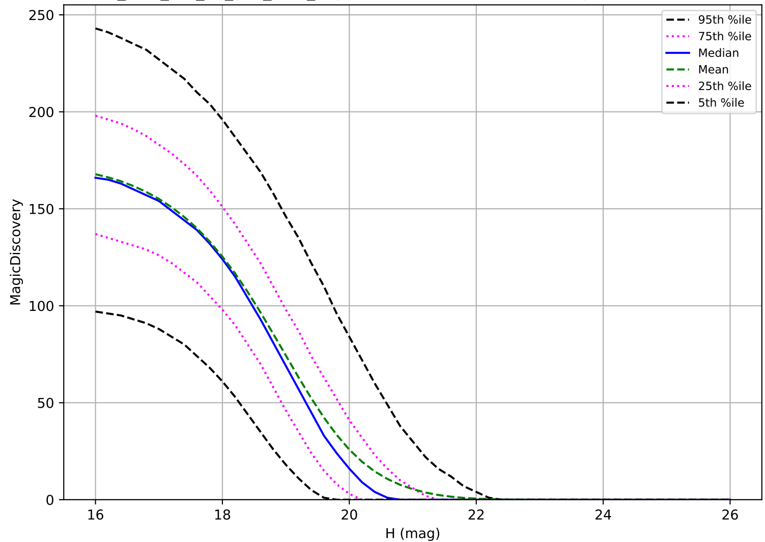
too_elab_r64_d2_griz_v3.4_10yrs: MBA 6 detections in 60 nights detection loss
