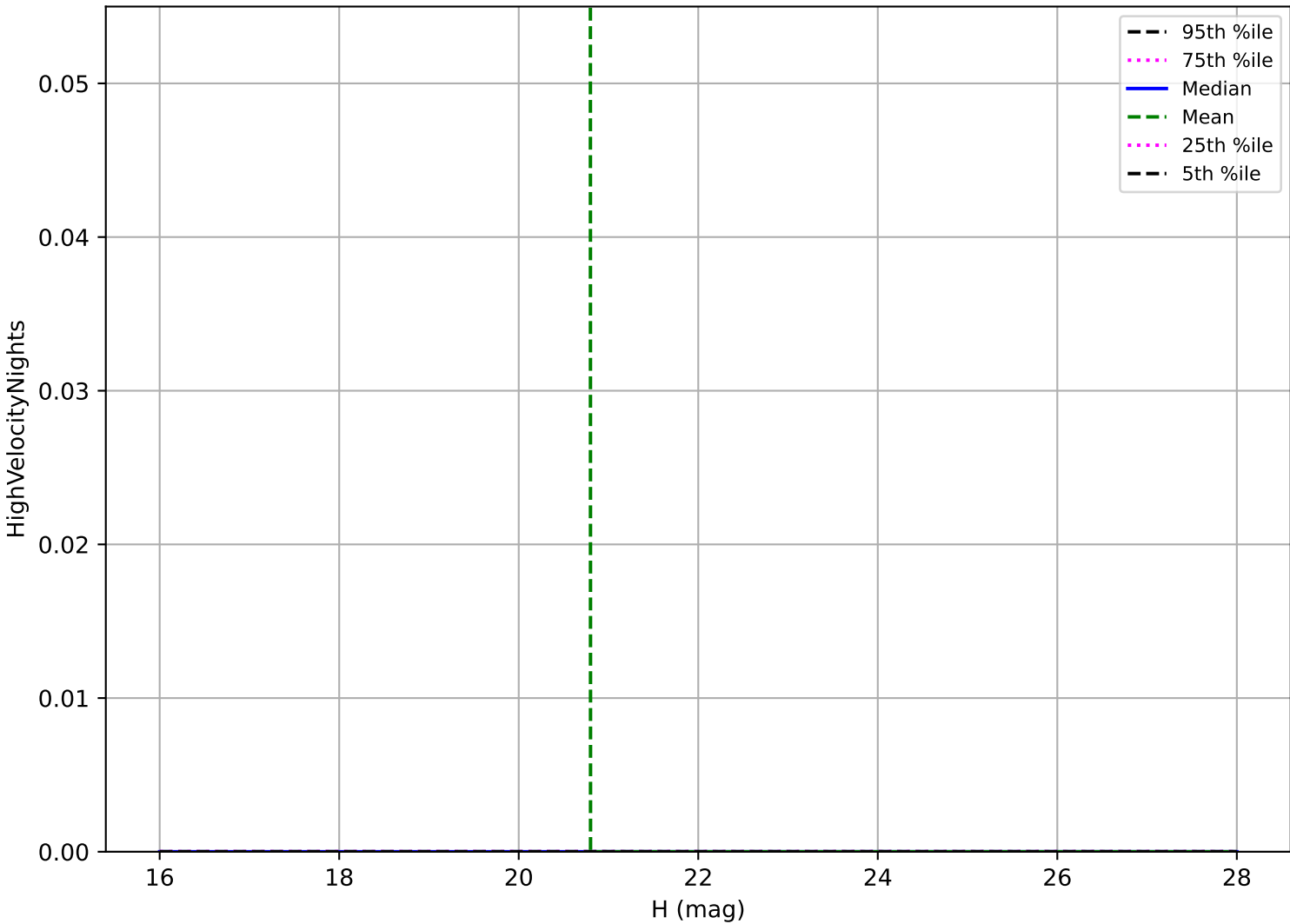
too_elab_r64_d2_griz_v3.4_10yrs: Vatira High velocity pair detection loss
