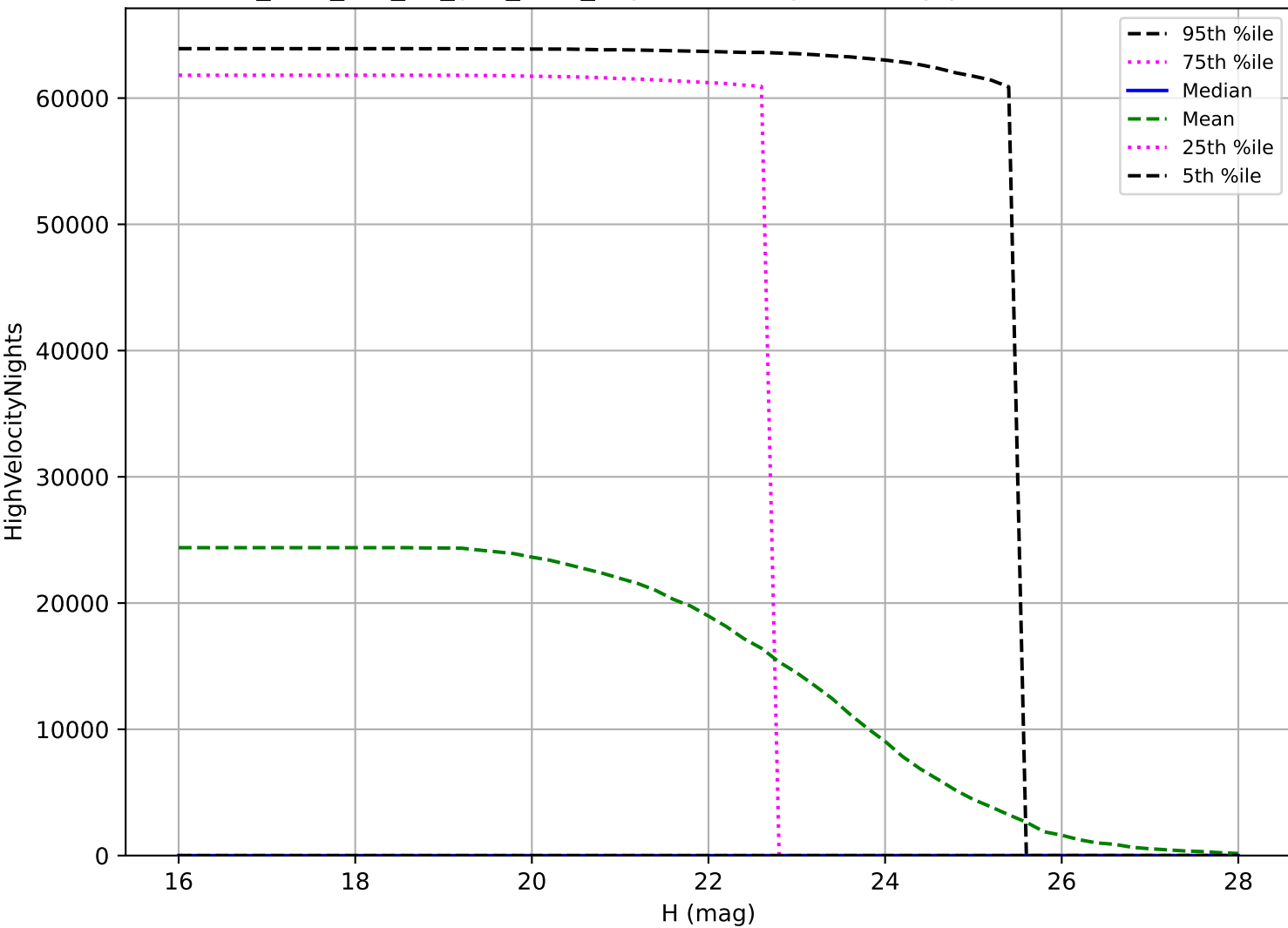
too_elab_r64_d2_griz_v3.4_10yrs: PHA High velocity pair detection loss
