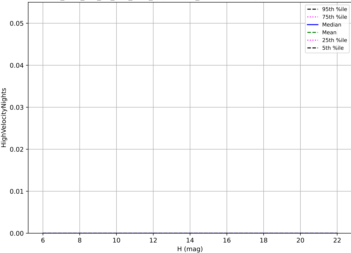
too_elab_r64_d2_griz_v3.4_10yrs: OCC_r5 High velocity pair detection loss
