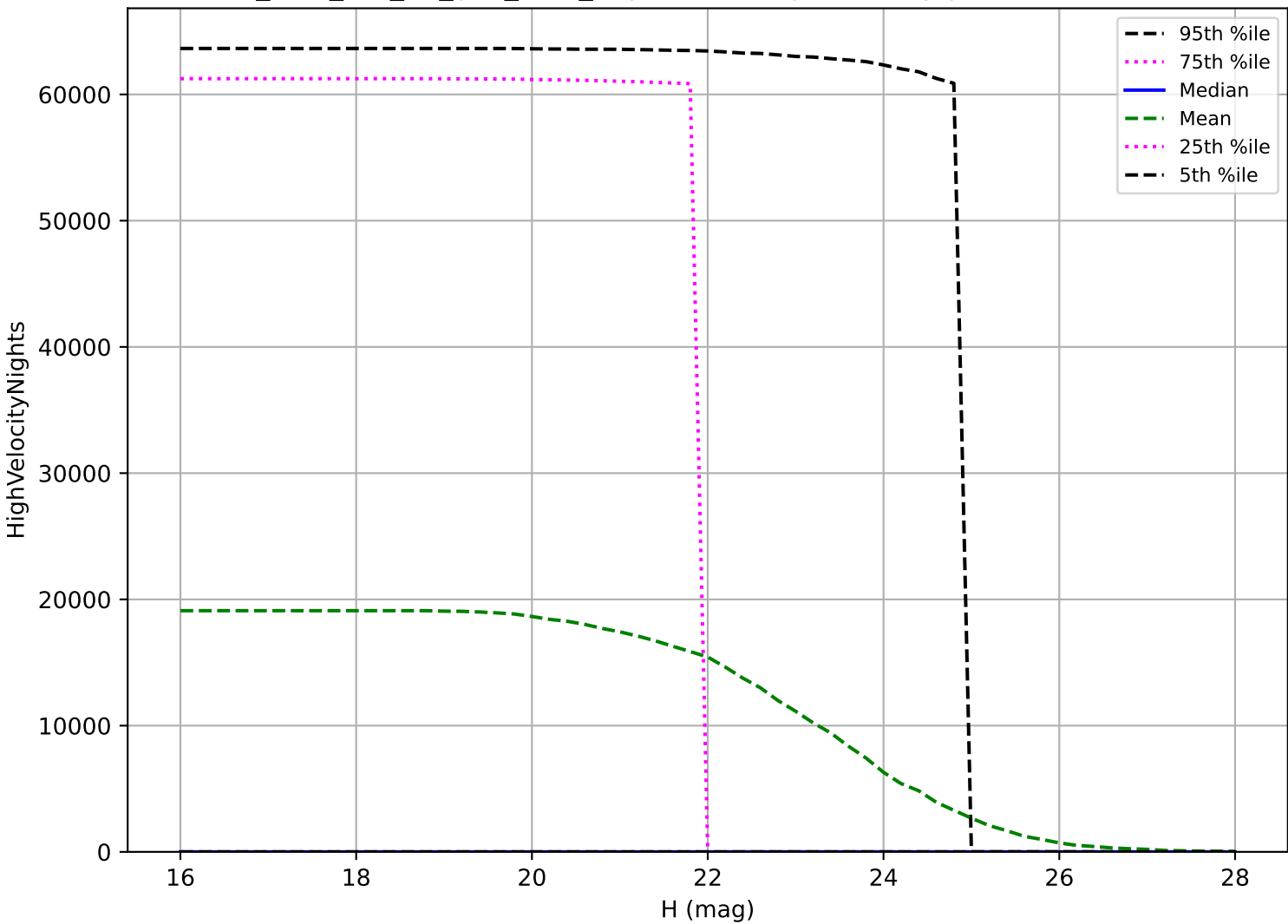
too_elab_r64_d2_griz_v3.4_10yrs: NEO High velocity pair detection loss
