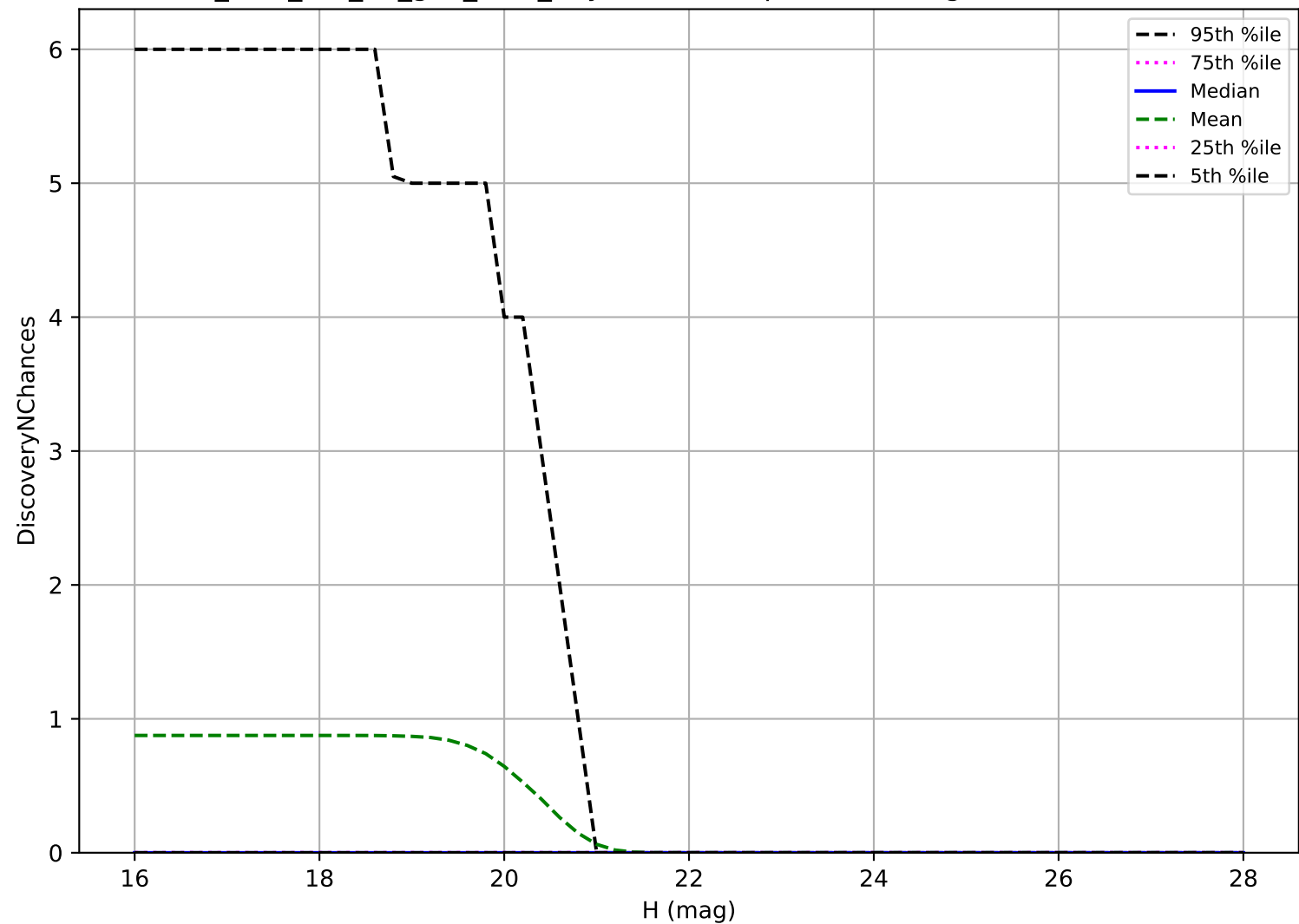
too_elab_r64_d2_griz_v3.4_10yrs: Vatira 3 pairs in 15 nights detection loss
