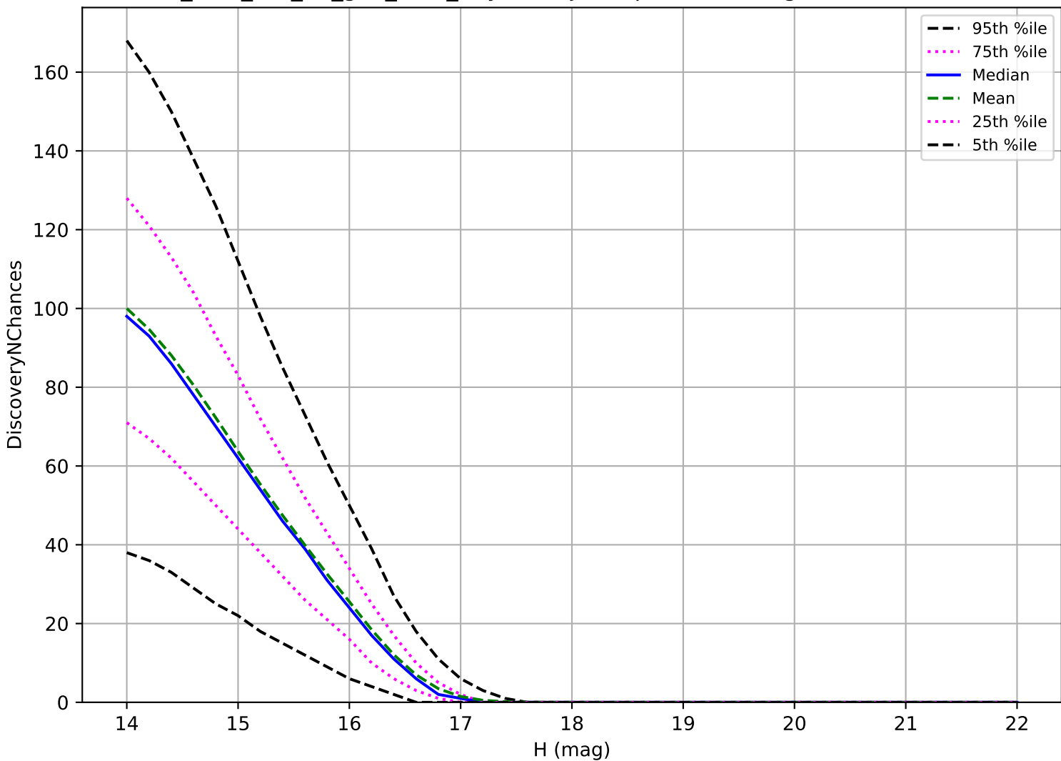
too_elab_r64_d2_griz_v3.4_10yrs: Trojan 3 pairs in 15 nights detection loss
