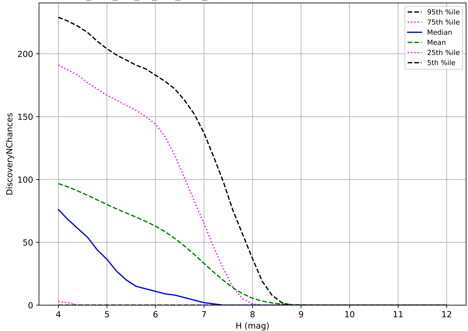
too_elab_r64_d2_griz_v3.4_10yrs: TNO 3 pairs in 15 nights detection loss
