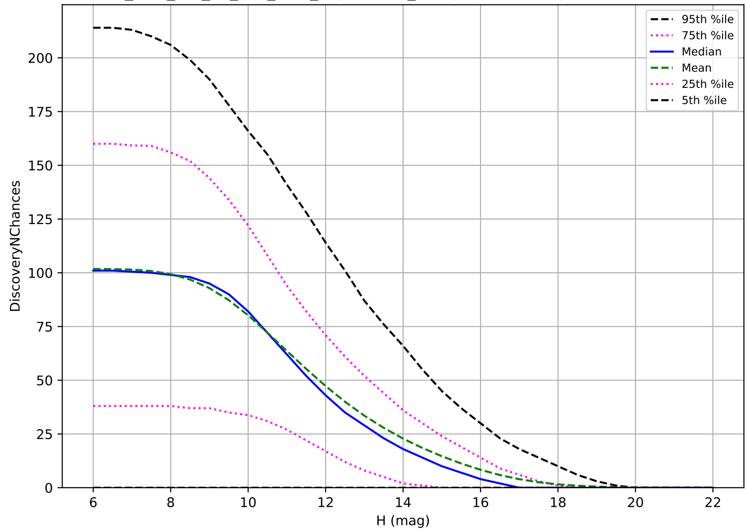
too_elab_r64_d2_griz_v3.4_10yrs: OCC_r5 3 pairs in 15 nights detection loss
