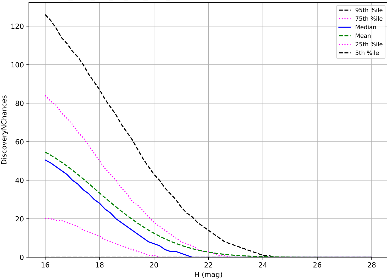
too_elab_r64_d2_griz_v3.4_10yrs: NEO 3 pairs in 15 nights detection loss
