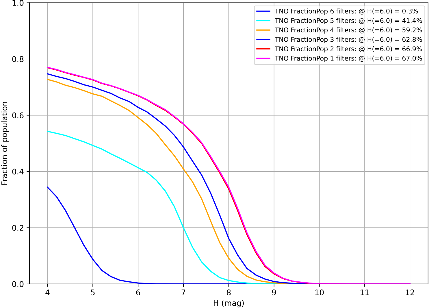
too_elab_r64_d2_griz_v3.4_10yrs: Fraction of population with colors in X filters TNO
