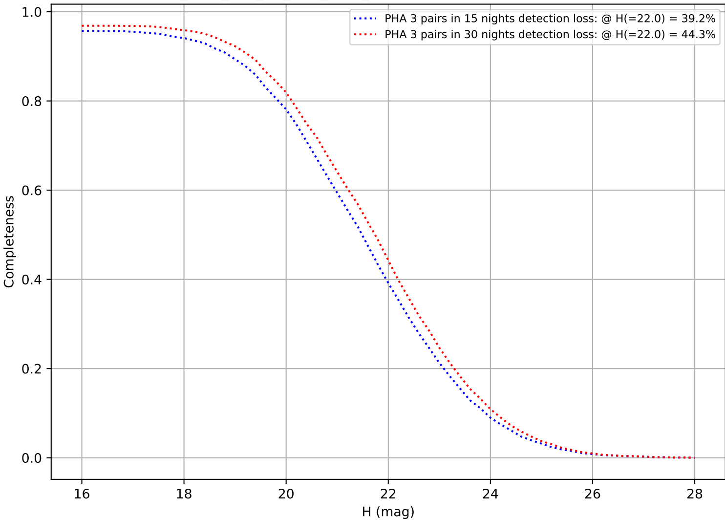
too_elab_r64_d2_griz_v3.4_10yrs: DifferentialCompleteness
