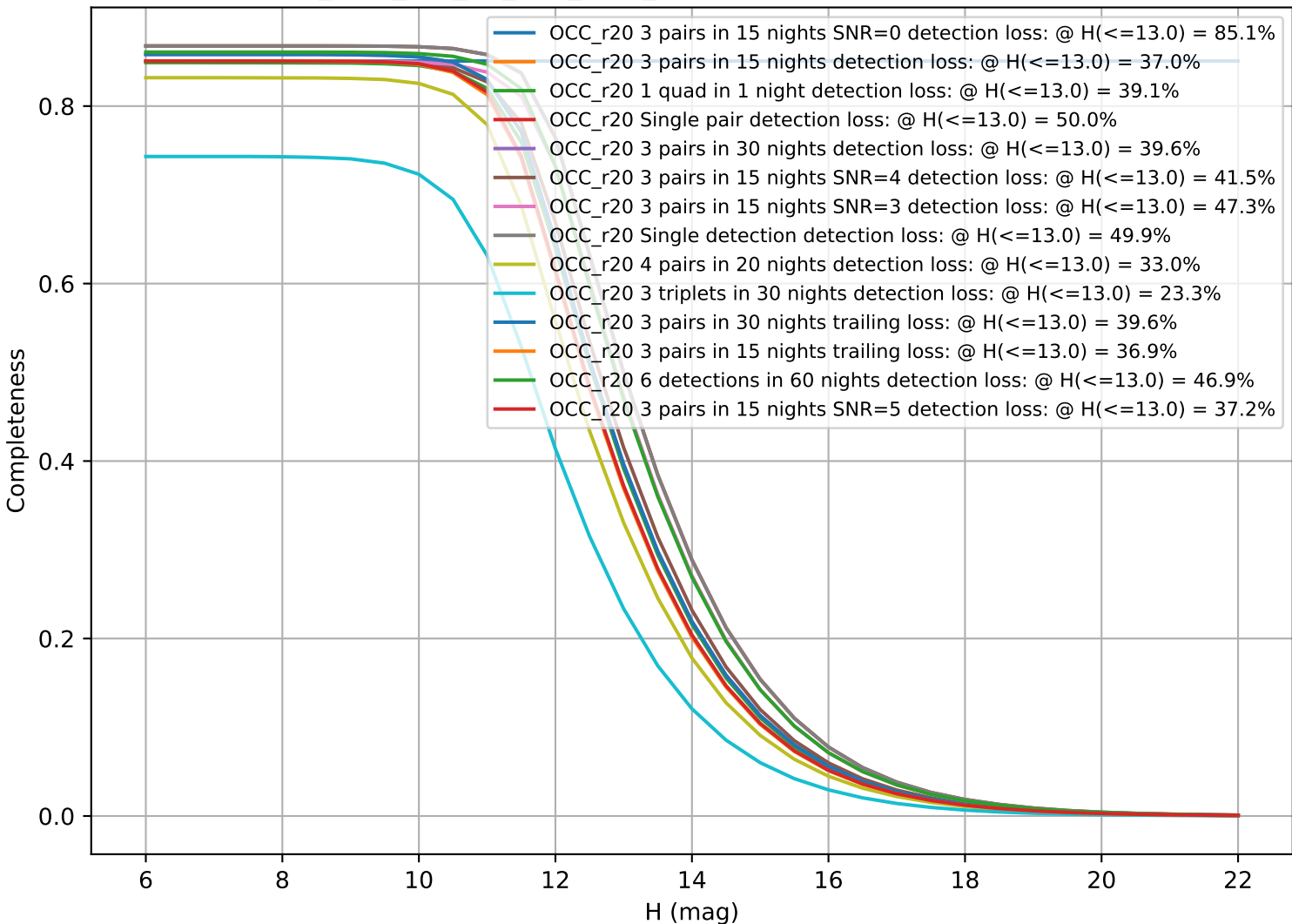
too_elab_r64_d2_griz_v3.4_10yrs: CumulativeCompleteness
