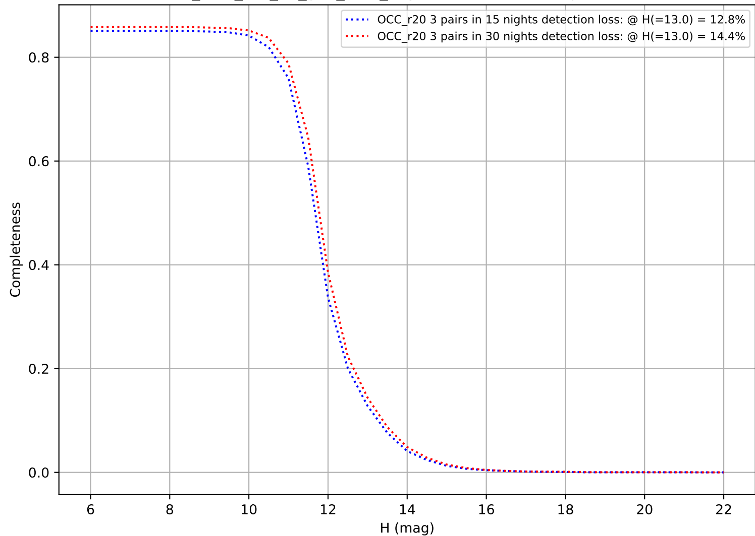
too_elab_r64_d2_griz_v3.4_10yrs: DifferentialCompleteness
