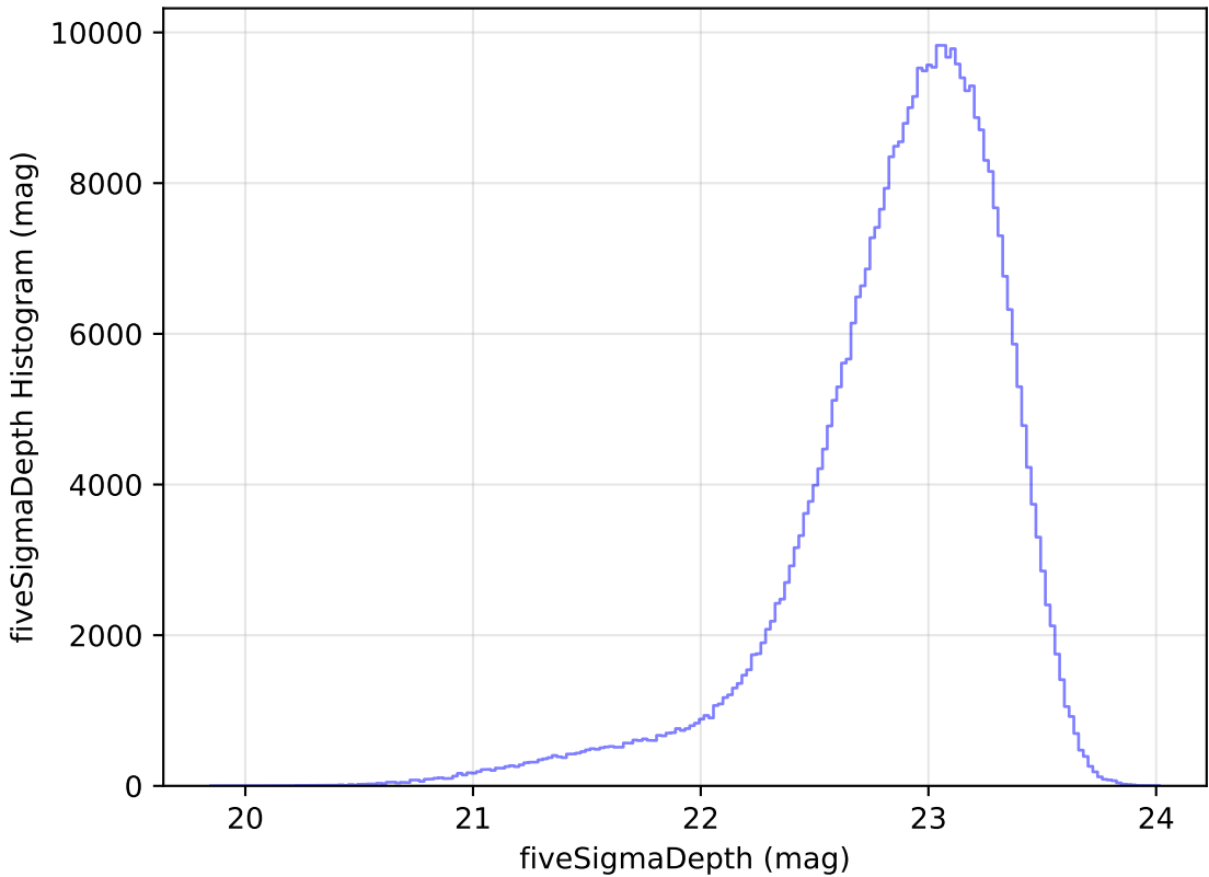
too_elab_r64_d2_griz_v3.4_10yrs z: fiveSigmaDepth Histogram
