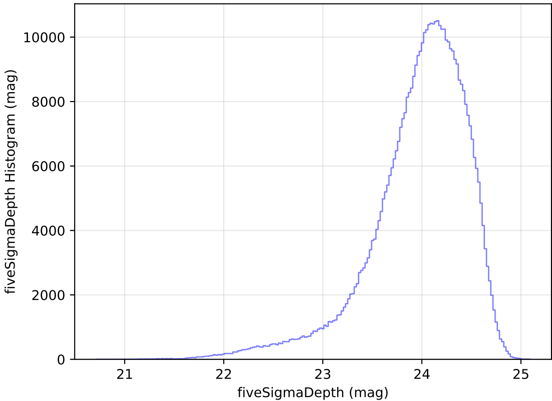
too_elab_r64_d2_griz_v3.4_10yrs r: fiveSigmaDepth Histogram
