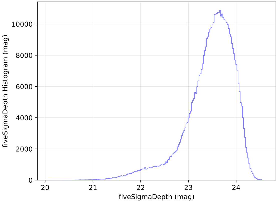
too_elab_r64_d2_griz_v3.4_10yrs i: fiveSigmaDepth Histogram
