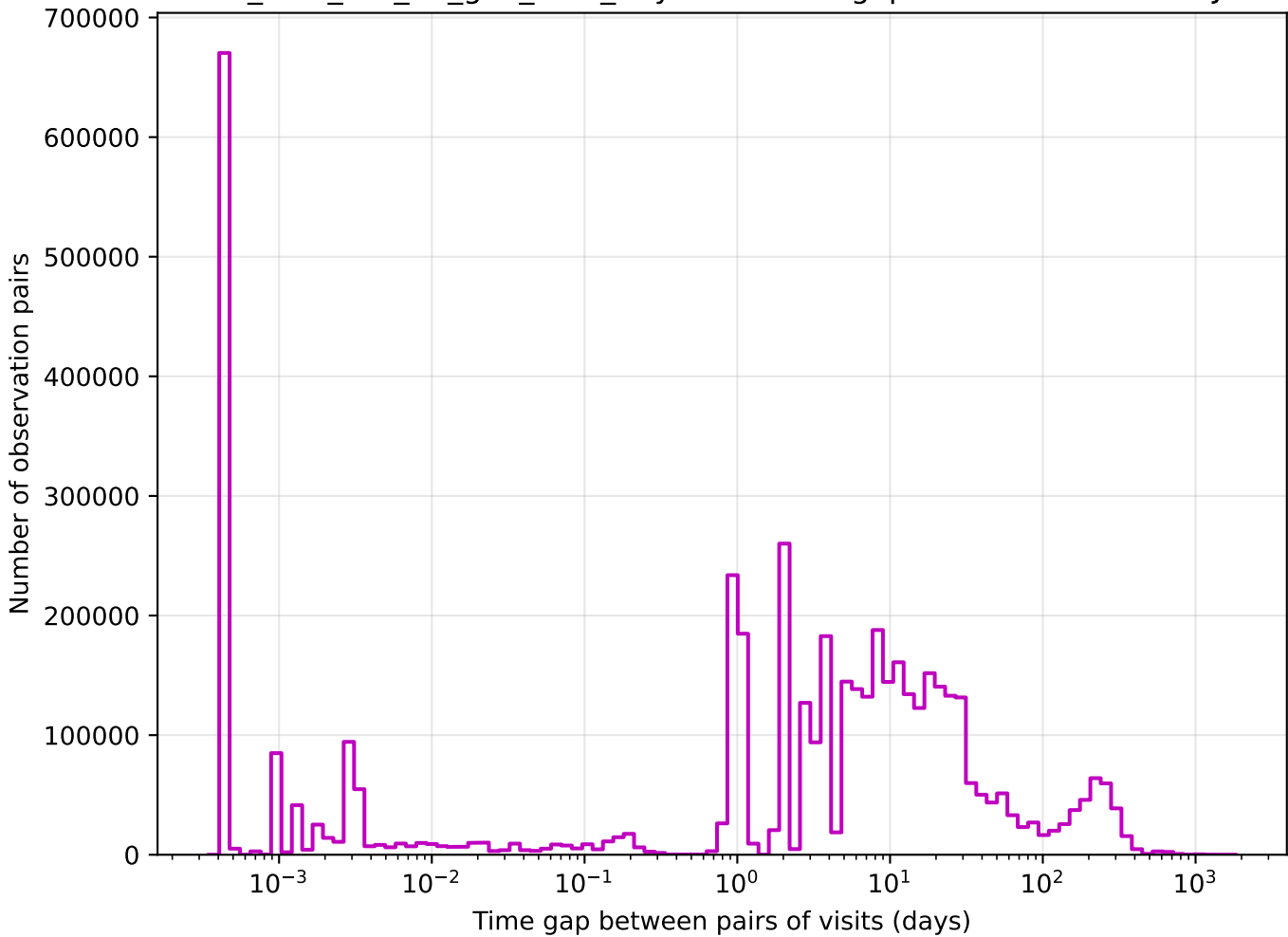
too_elab_r64_d2_griz_v3.4_10yrs z band: Tgaps observationStartMJD
