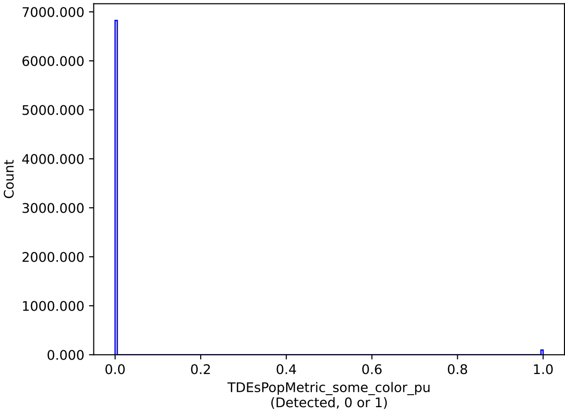
too_elab_r64_d2_griz_v3.4_10yrs : TDEsPopMetric_some_color_pu
