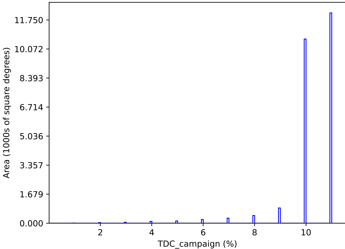
too_elab_r64_d2_griz_v3.4_10yrs : TDC_campaign
