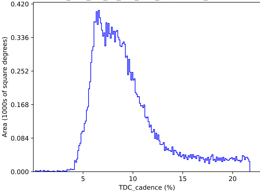
too_elab_r64_d2_griz_v3.4_10yrs : TDC_cadence
