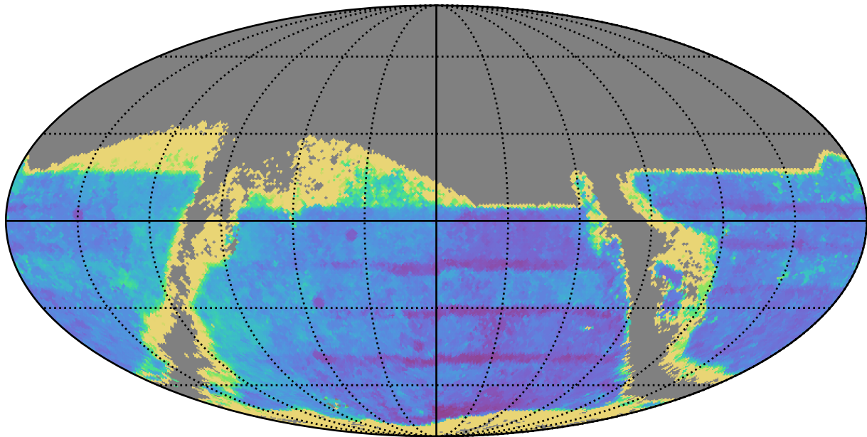
too_elab_r64_d2_griz_v3.4_10yrs : TDC_accuracy
