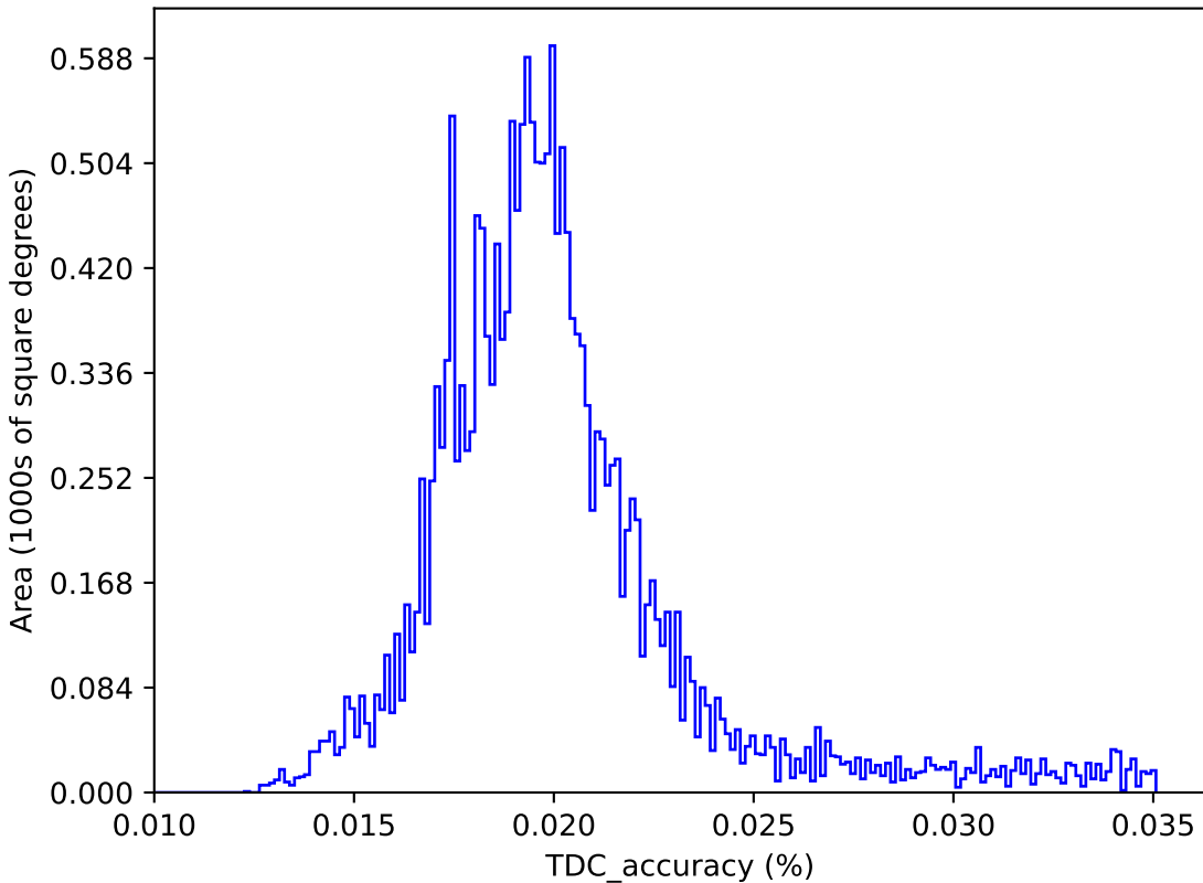
too_elab_r64_d2_griz_v3.4_10yrs : TDC_accuracy
