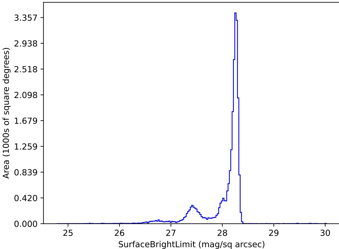
too_elab_r64_d2_griz_v3.4_10yrs y: SurfaceBrightLimit
