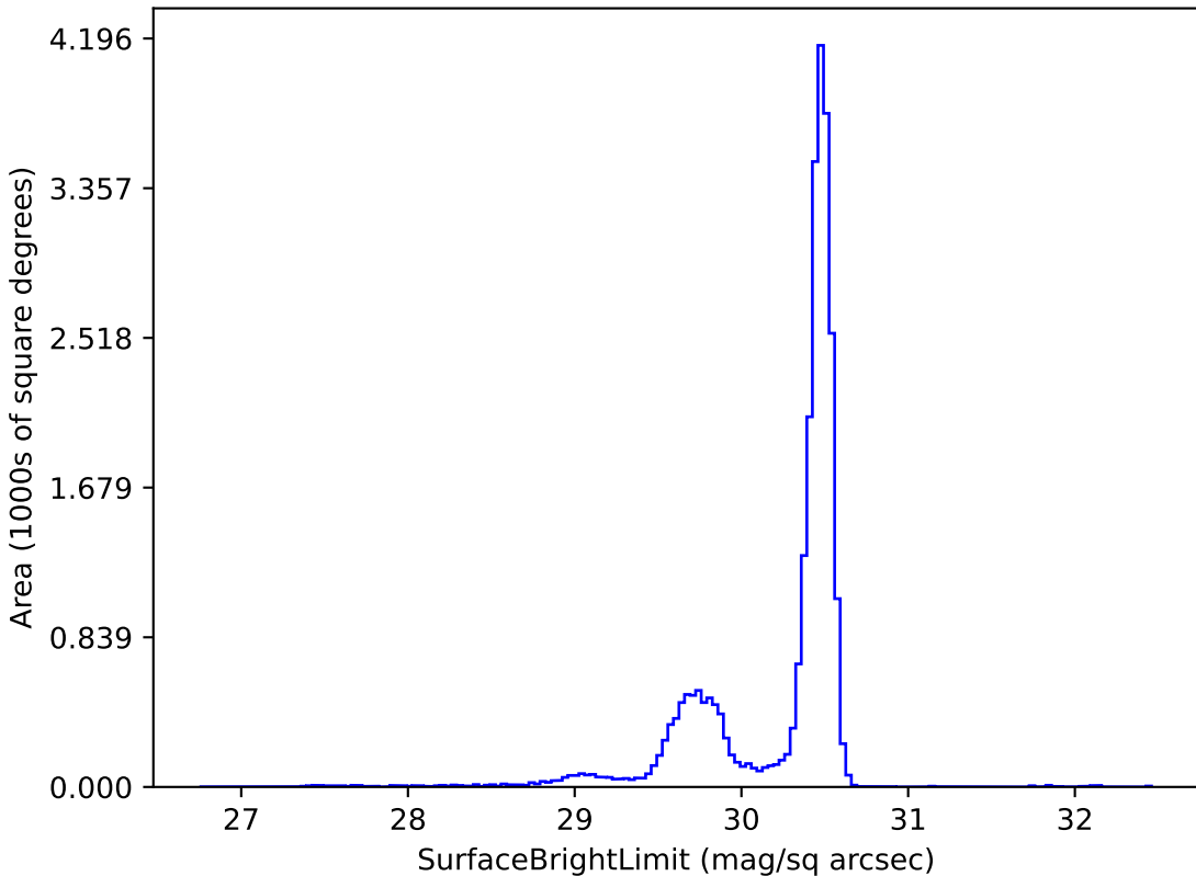
too_elab_r64_d2_griz_v3.4_10yrs r: SurfaceBrightLimit
