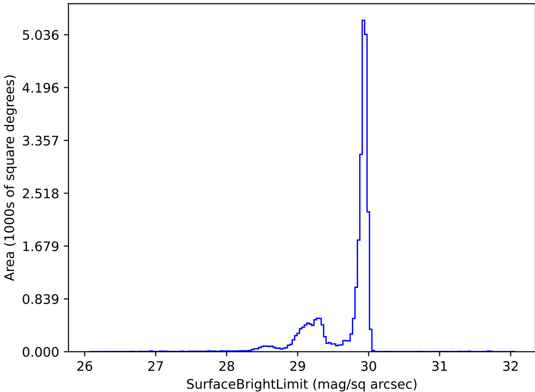
too_elab_r64_d2_griz_v3.4_10yrs i: SurfaceBrightLimit
