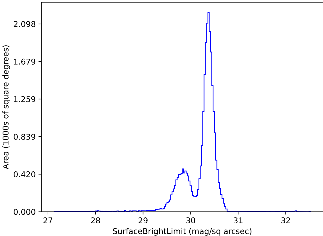
too_elab_r64_d2_griz_v3.4_10yrs g: SurfaceBrightLimit
