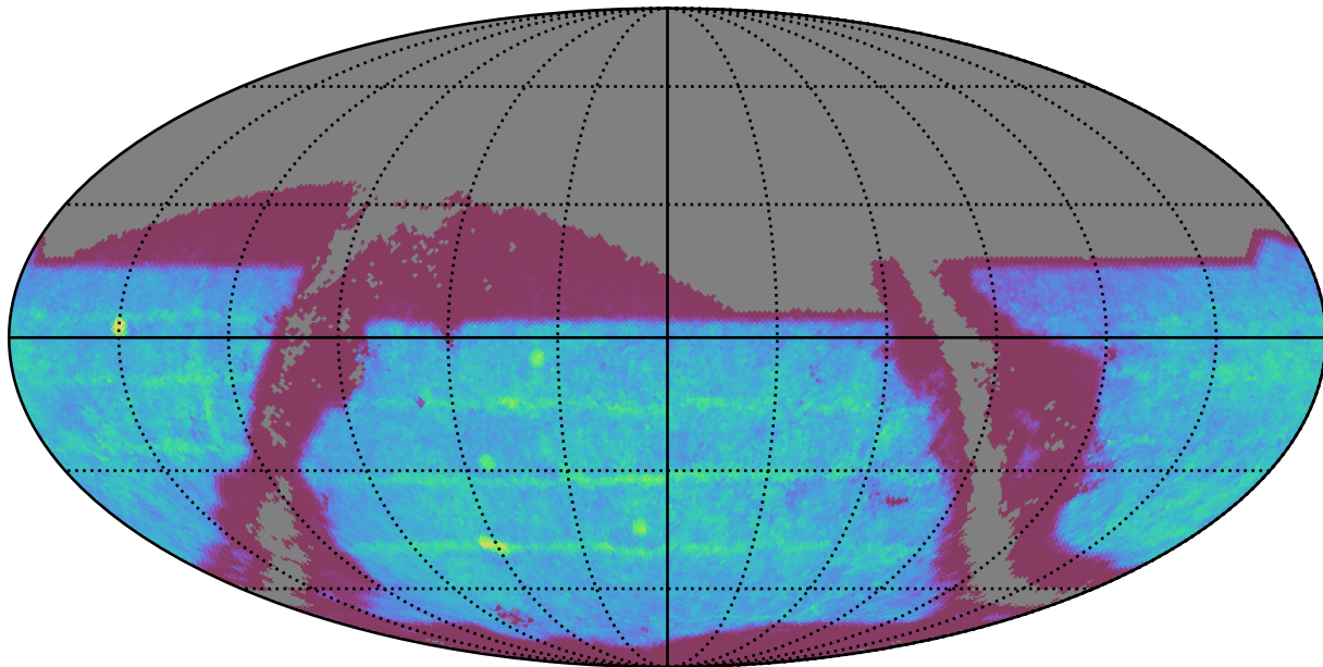
too_elab_r64_d2_griz_v3.4_10yrs : SNSLMetric
