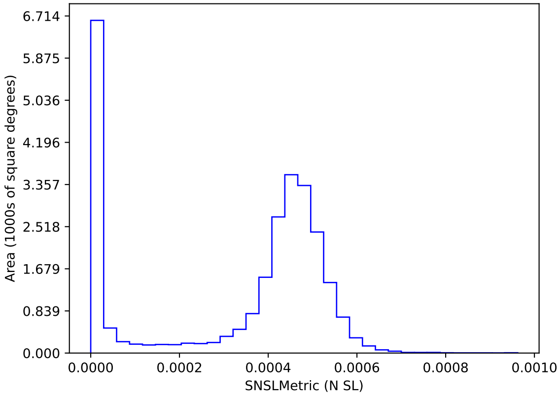
too_elab_r64_d2_griz_v3.4_10yrs : SNSLMetric
