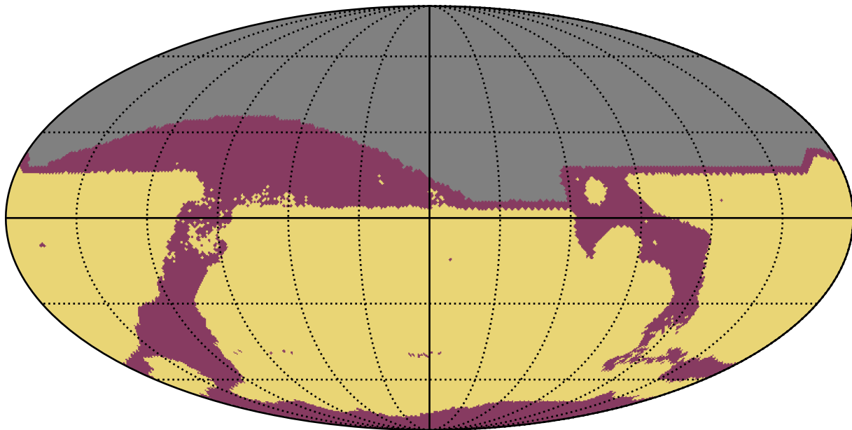
too_elab_r64_d2_griz_v3.4_10yrs : RapidRevisits
