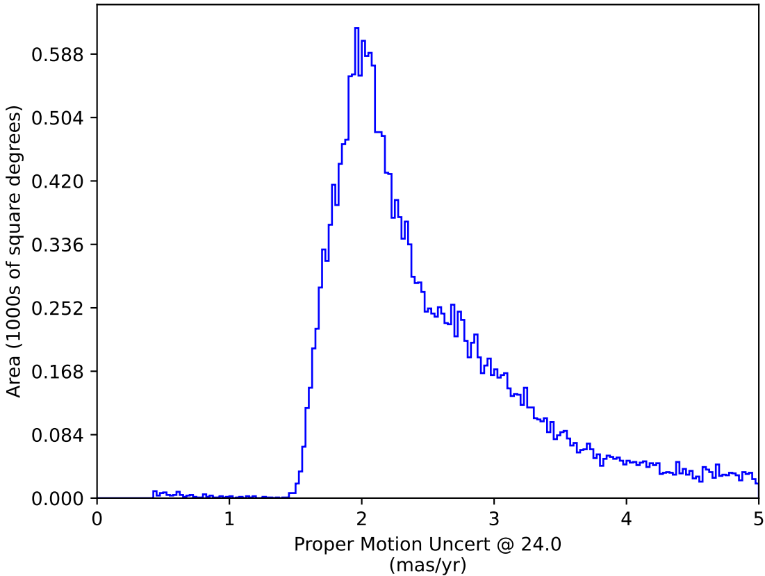
too_elab_r64_d2_griz_v3.4_10yrs : Proper Motion Uncert @ 24.0
