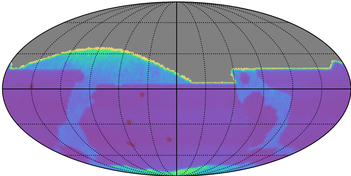
too_elab_r64_d2_griz_v3.4_10yrs : Proper Motion Uncert @ 20.5
