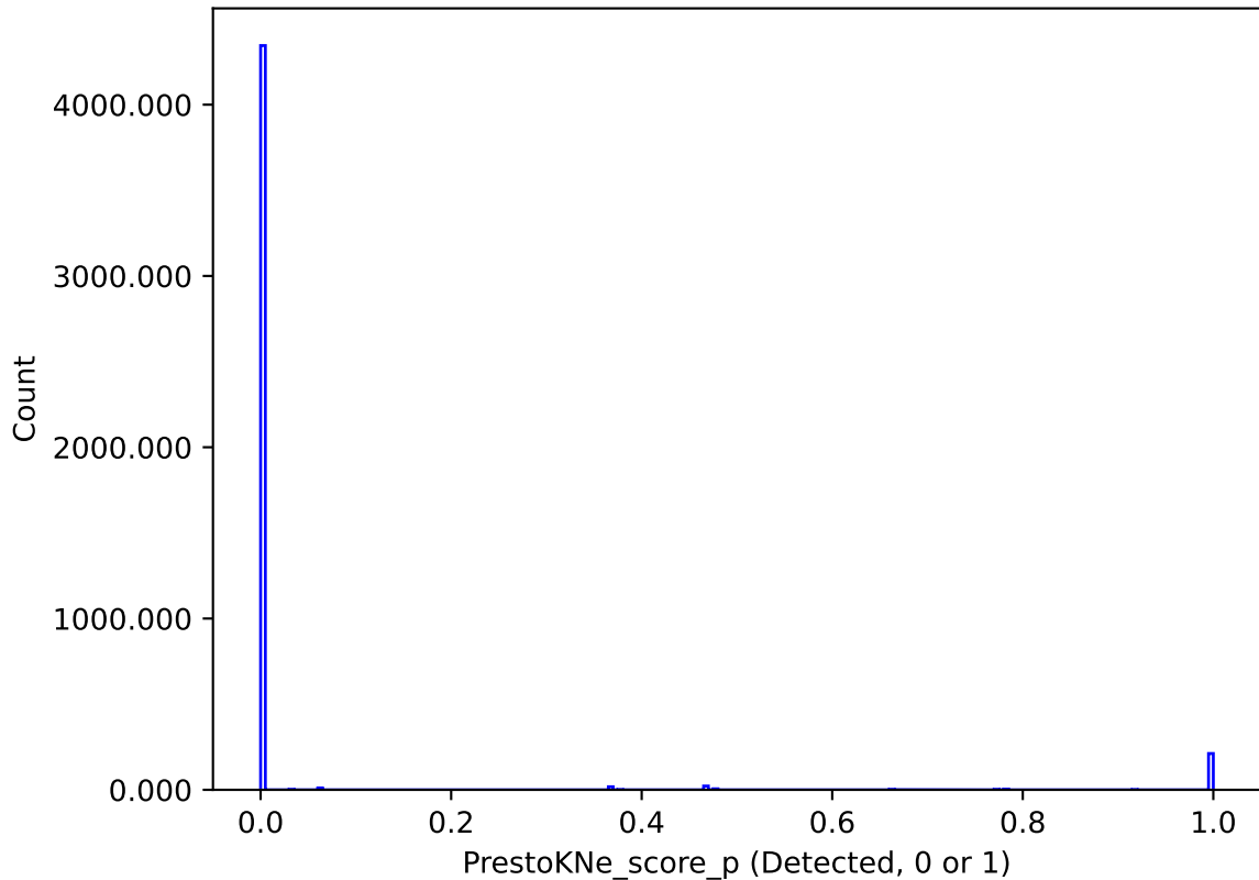
too_elab_r64_d2_griz_v3.4_10yrs : PrestoKNe_score_p
