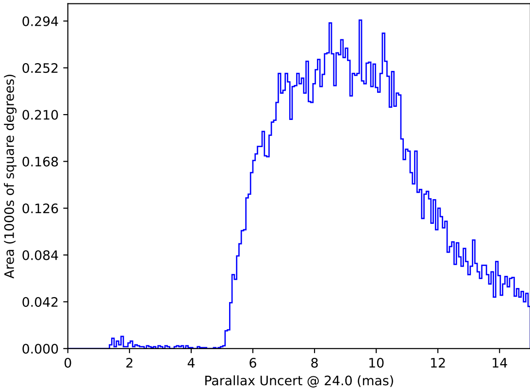
too_elab_r64_d2_griz_v3.4_10yrs : Parallax Uncert @ 24.0
