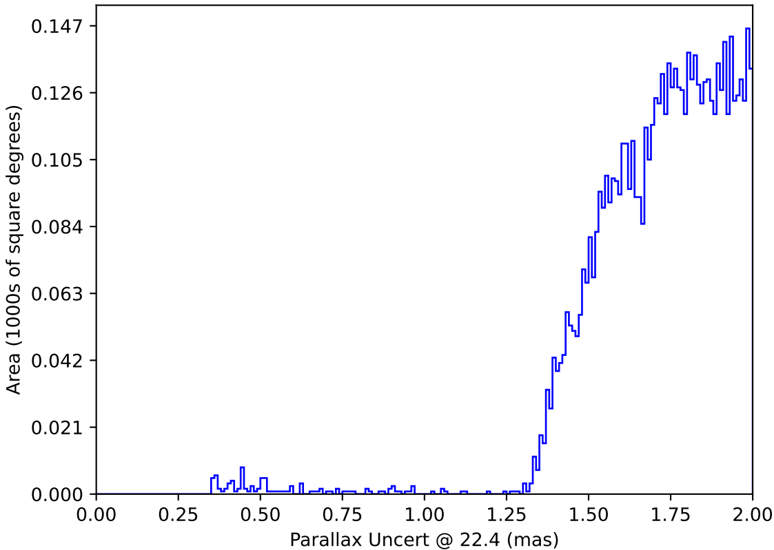
too_elab_r64_d2_griz_v3.4_10yrs : Parallax Uncert @ 22.4
