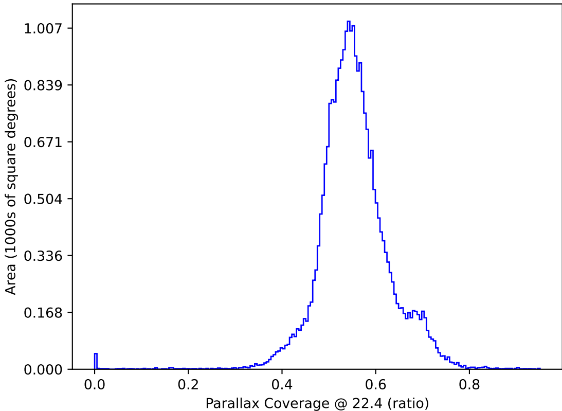
too_elab_r64_d2_griz_v3.4_10yrs : Parallax Coverage @ 22.4
