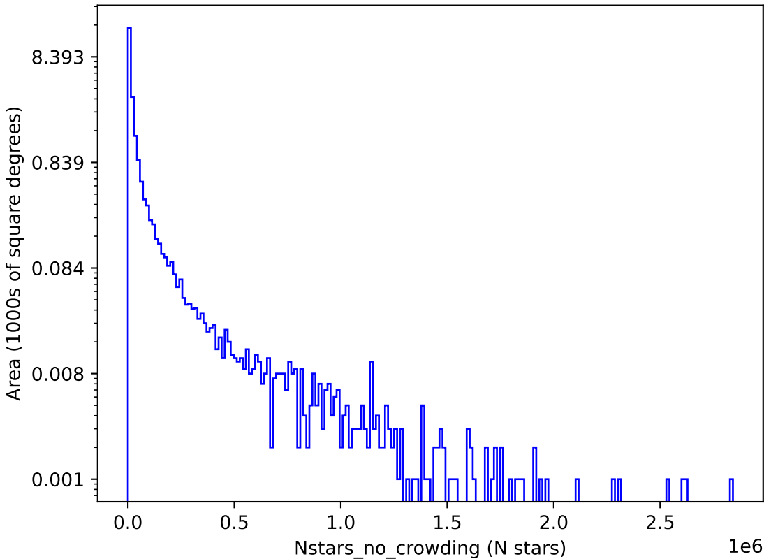
too_elab_r64_d2_griz_v3.4_10yrs u: Nstars_no_crowding
