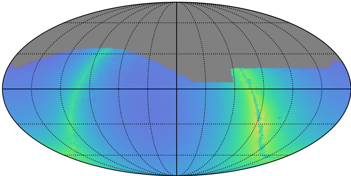
too_elab_r64_d2_griz_v3.4_10yrs i: Nstars_no_crowding
