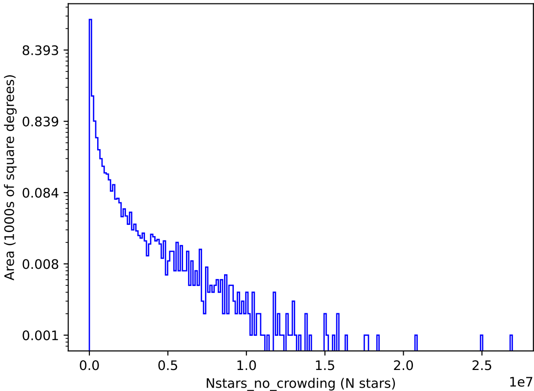
too_elab_r64_d2_griz_v3.4_10yrs i: Nstars_no_crowding
